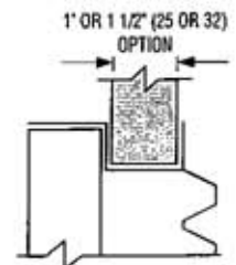
MODEL 08SH HINGED DOOR (WITH CAMLOCK CLOSURE)
