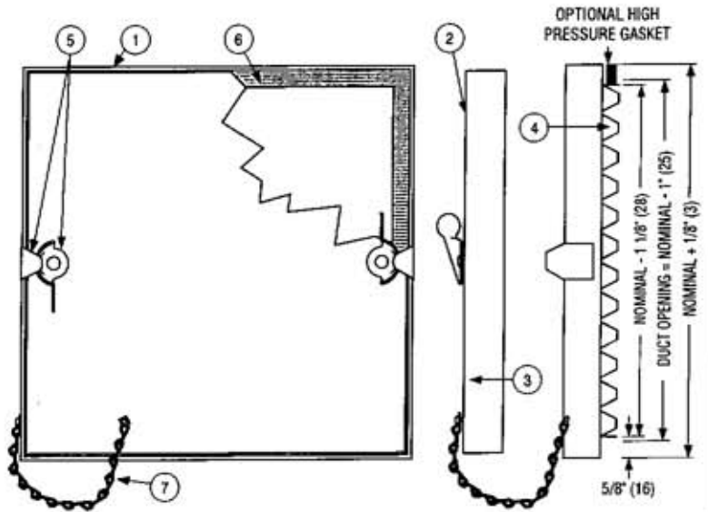
MODEL 08SCL REMOVABLE DOOR (PAIRED CAMLOCKS)
